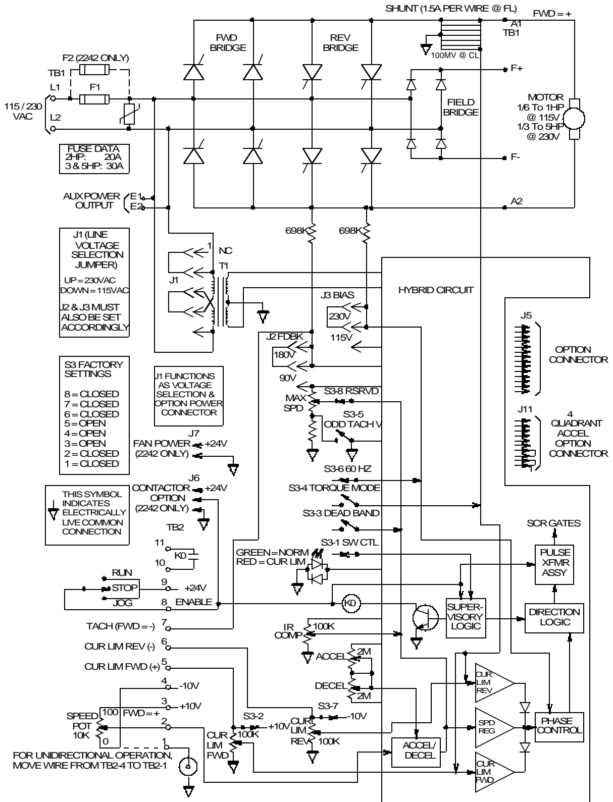
FIGURE 9-1. FUNCTIONAL SCHEMATIC, SERIES 2230/2240 CONTROLLERS
