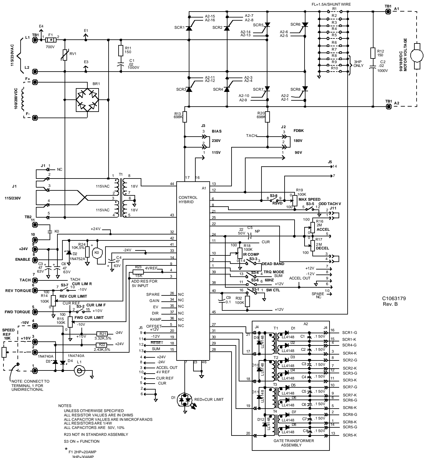
FIGURE 9-2. SCHEMATIC, MODEL 2231, 2232, 2235, AND 2236 CONTROLLERS
